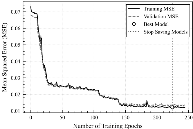
Learning Curve of TCSA-LSTM Model for SolarPlant-2 (Gyeongju)
